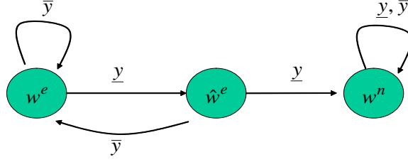
Figure 4: Forgiving grim trigger where two successive realizations of \underline{y} lead to w^n .
