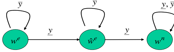
Figure 3: Forgiving grim trigger where any two realizations of \underline{y} lead to w^n .
