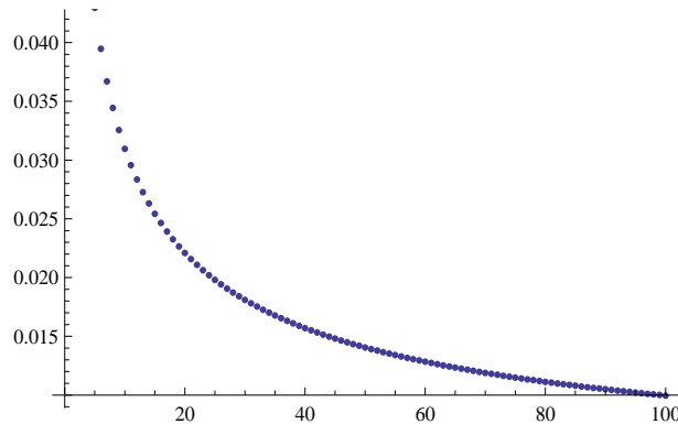
FIGURE 1. Horizontal axis: Market size q . Vertical axis: RP_b^q(\pi) . Note that the assignment coincides with PS (and hence is ordinally efficient) if RP_b^q(\pi) = 0 .
