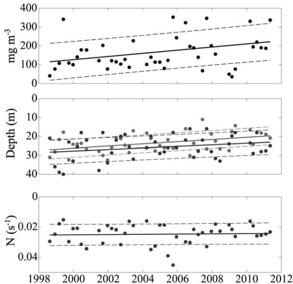
Fig. 11. (A) Integrated Chl a , (B) depth of mixed layer and Chl a center of mass, and (C) mean stratification at base of mixed layer from 1998–2012. Solid lines represent linear least-squares best fit regression. Dashed lines show 95% confidence intervals of the fits.
