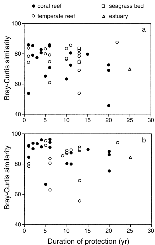
FIG. 5. Bray-Curtis percentage similarity in (a) species and (b) trophic group composition of fish assemblages between no-take reserves of varying ages (i.e., duration of protection, in years) and reference conditions.
