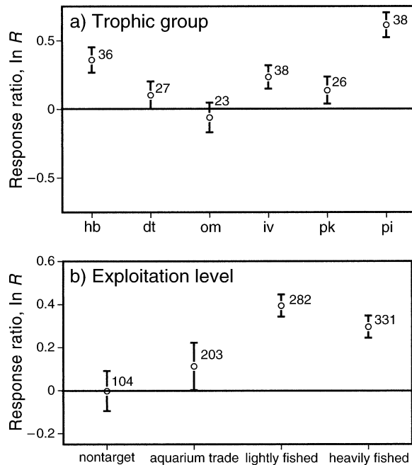
FIG. 3. Results of meta-analyses of the response ratios ( \ln R ) for (a) each of six trophic groups (hb, herbivores; dt, detritivores; om, omnivores; iv, invertebrate feeders; pk, planktivores; pi, piscivores) and (b) four exploitation levels (nontarget species, species targeted by the aquarium trade, and species lightly or heavily fished). Mean response ratios, weighted by sampling variances, are reported for each category. Bars represent 95% CI. When confidence intervals do not overlap 0, weighted averages are considered significantly different from 0. The number of comparisons within each category is reported to the right of each mean.
