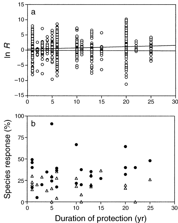
FIG. 1. (a) Response ratios ( \ln R , calculated as the natural log of the ratios between abundances within reserves and in reference conditions) of individual species. (b) Percentages of species within each study exhibiting positive responses (solid circles; \ln R \geq 0.69 , see Methods: Variation and correlates of species responses to protection ) or negative responses (open triangles; \ln R \leq -0.69 ) to protection in reserves ranging from one to 25 years of protection.
