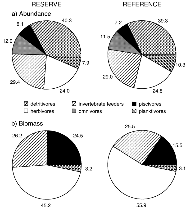
FIG. 6. Percentages of (a) total fish abundances and (b) biomass in different trophic groups. Percentages are weighted means of values from (a) 38 abundance comparisons between protected and fished areas from 20 individual studies and (b) 10 biomass comparisons from five studies.
