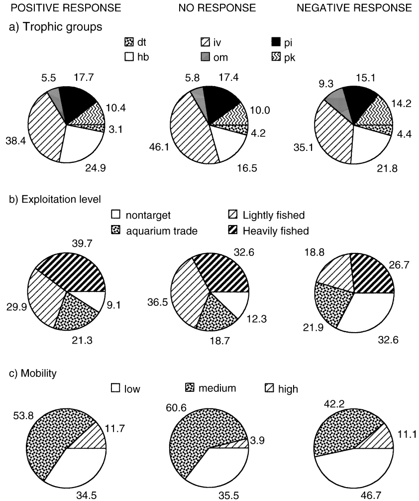
FIG. 2. Percentages of species exhibiting positive ( \ln R \geq 0.69 ), intermediate (i.e., no response, -0.69 < \ln R < 0.69 ), and negative ( \ln R \leq -0.69 ) responses to protection in different (a) trophic groups (hb, herbivores; dt, detritivores; om, omnivores; iv, invertebrate feeders; pk, planktivores; pi, piscivores), (b) exploitation levels, and (c) adult mobility categories.
