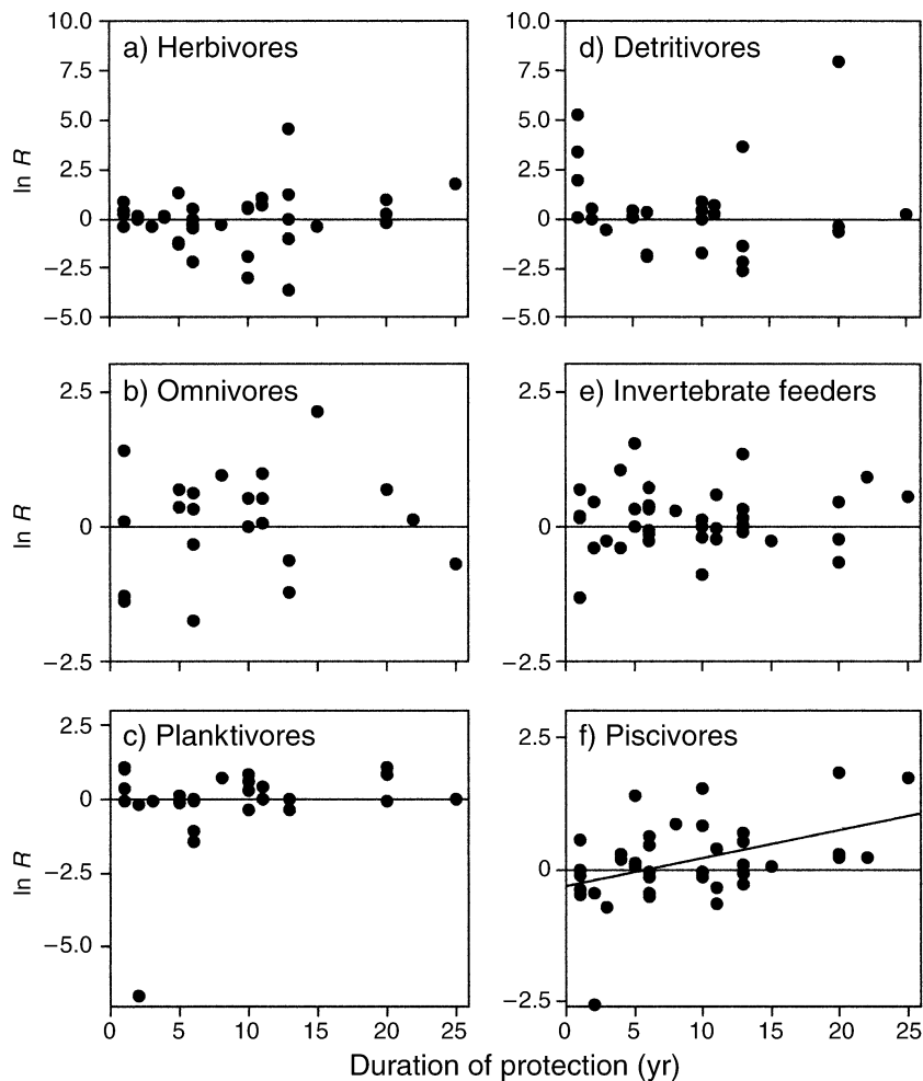
FIG. 4. Response ratios ( \ln R ) vs. duration of protection for each of six trophic groups. A statistically significant temporal trend was found only for piscivores.
