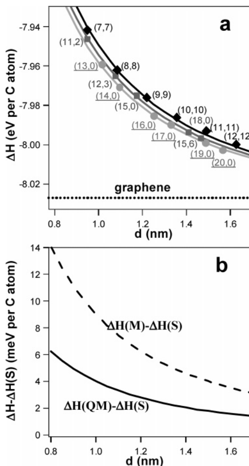
Figure 4. (a) Density functional theory (DFT) calculations of the atomic heat of formation ( \Delta H ) versus tube diameter ( d ) for various M-, QM-, and S-SWNTs (denoted by symbols); the three solid lines are \sim 1/d^2 fits for the formation energy, relative to graphene, for the three types of tubes. (b) Difference in formation energies between M- and S-SWNTs (dashed line) and QM- and S-SWNTs (solid line), versus tube diameter d ; note that, for a SWNT with d \approx 1 nm, although the per atom energy gain for a semiconductor is small (a few meV), the energy cost for adding a “belt” of atoms (extending the tube length by one C–C bond length) for the S-SWNT is lower than that for a M-SWNT (by \sim 0.15 eV), which is quite substantial ( k_B T \approx 0.07 eV at 600 °C). This energy is relevant, because SWNT growth from a seed particle occurs via supersaturation and precipitation of C atoms around the particle circumference.
