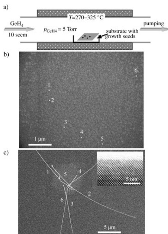
Figure 1. One-to-one growth of 20-nm GeNWs. a) Schematic of the LPCVD setup (sccm = standard cubic centimeters per minute), b) SEM image of six gold nanoparticles ( d \approx 20 nm) as growth seeds, and c) SEM image of the six GeNWs grown from the gold seeds labeled in (b). (The inset shows a high-resolution transmission electron microscopy image of a single-crystalline GeNW grown under the same conditions as those shown in the main panel).
