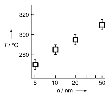
Figure 3. Size-dependent conditions for the growth of nanowires. A plot of the optimum temperature ( T ) for growth of the GeNW as a function of the size of the gold particle seeds, and hence the size of the nanowire, by CVD under a fixed partial pressure of 5 Torr of germane. For each particle size, the optimum growth temperature is denoted by a hollow square and the error bars span less than 10 °C.
