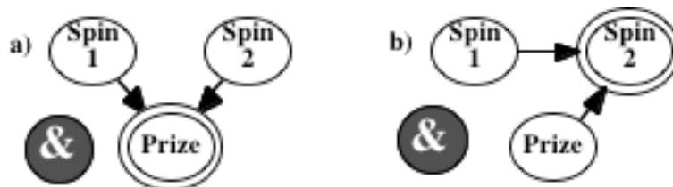
Figure 2. Different models for a coin spinning contest
