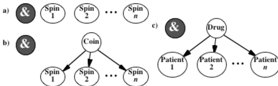
Figure 5. Repeated trials that are conditionally irrelevant
