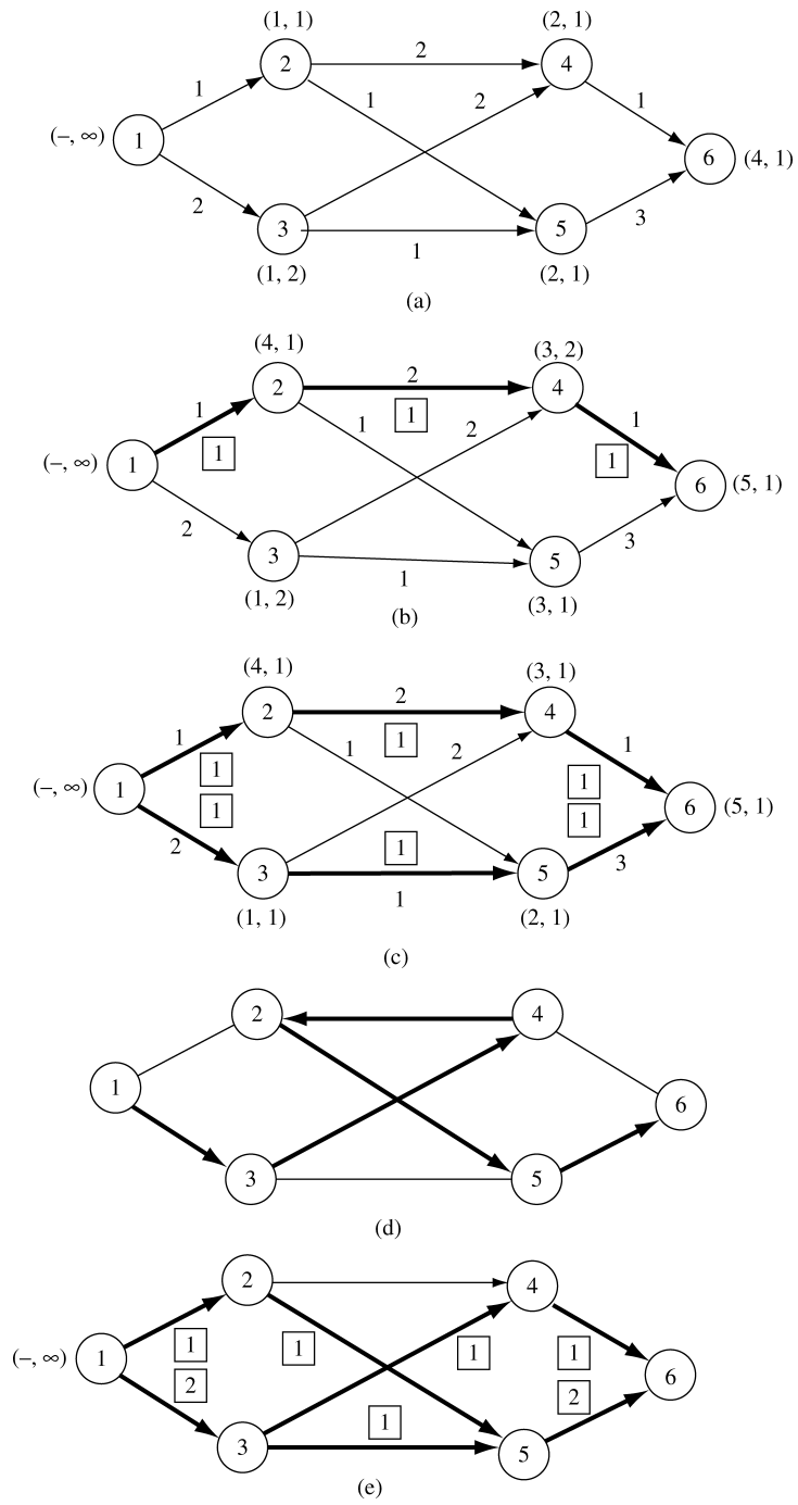
Fig. 4.4 Example of maximal flow problem
