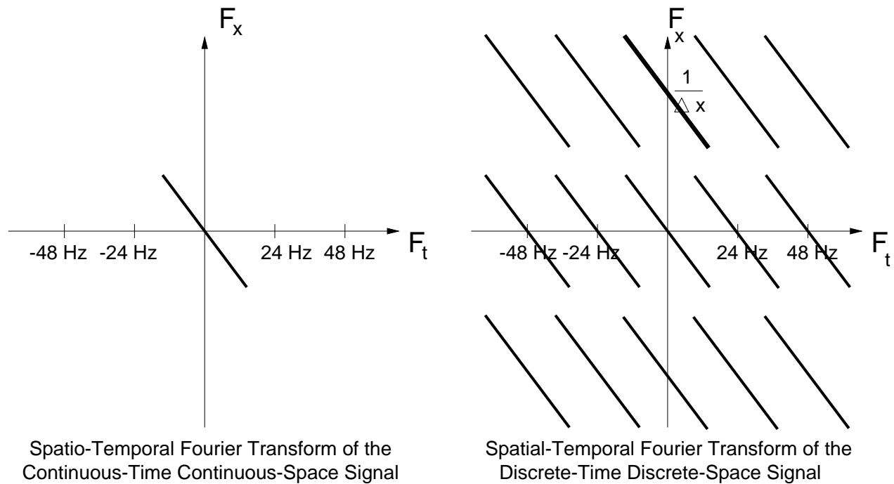
Figure 2: Spatio-temporal Fourier transform of sampled signal.
