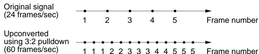
Figure 1: 3:2 pulldown
