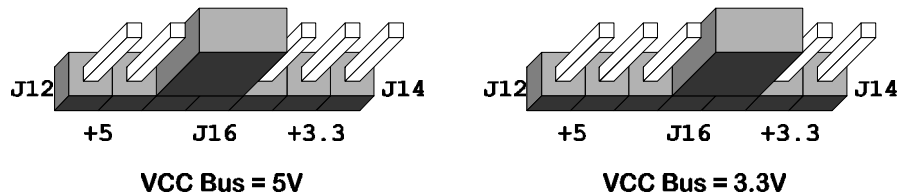
• Figure 4: Shunt placement for setting the VCC bus voltage..
